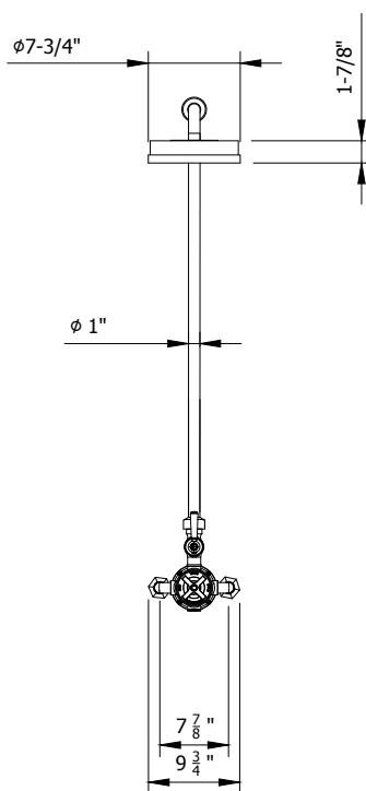
Waldorf Exposed Thermostatic Shower Set US-WF_SHOWER
