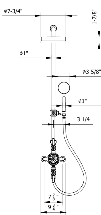
Waldorf Exposed Thermostatic Shower Set US-WF_SLIDER
